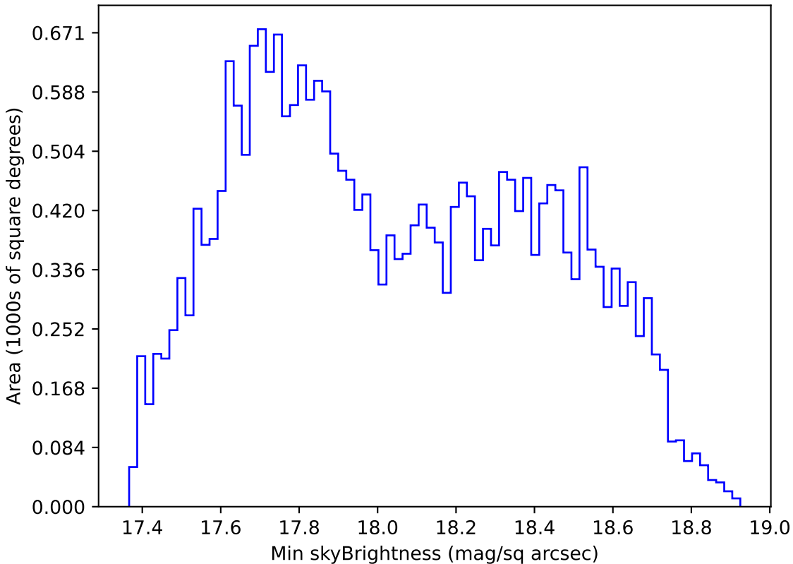
all_long_v3.4_10yrs All sky i band: Min skyBrightness
