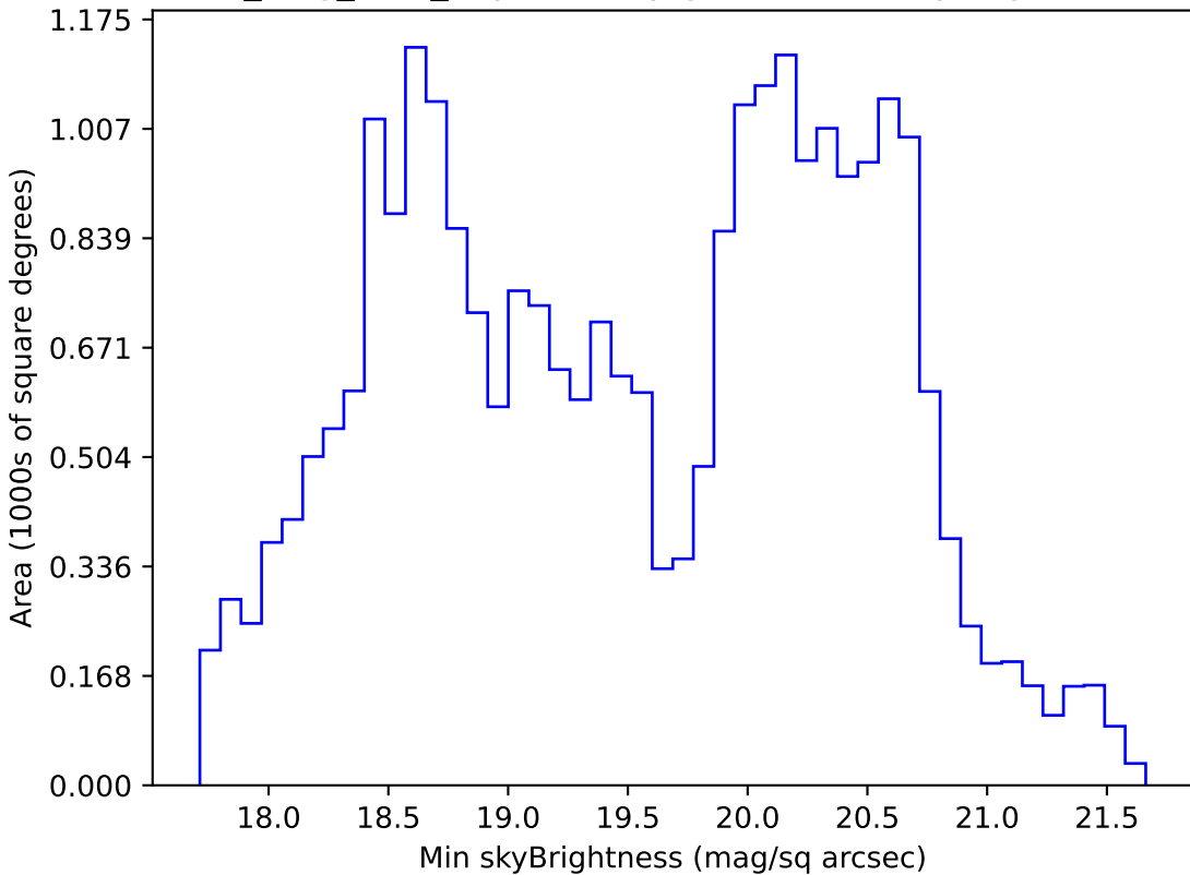
all_long_v3.4_10yrs All sky g band: Min skyBrightness
