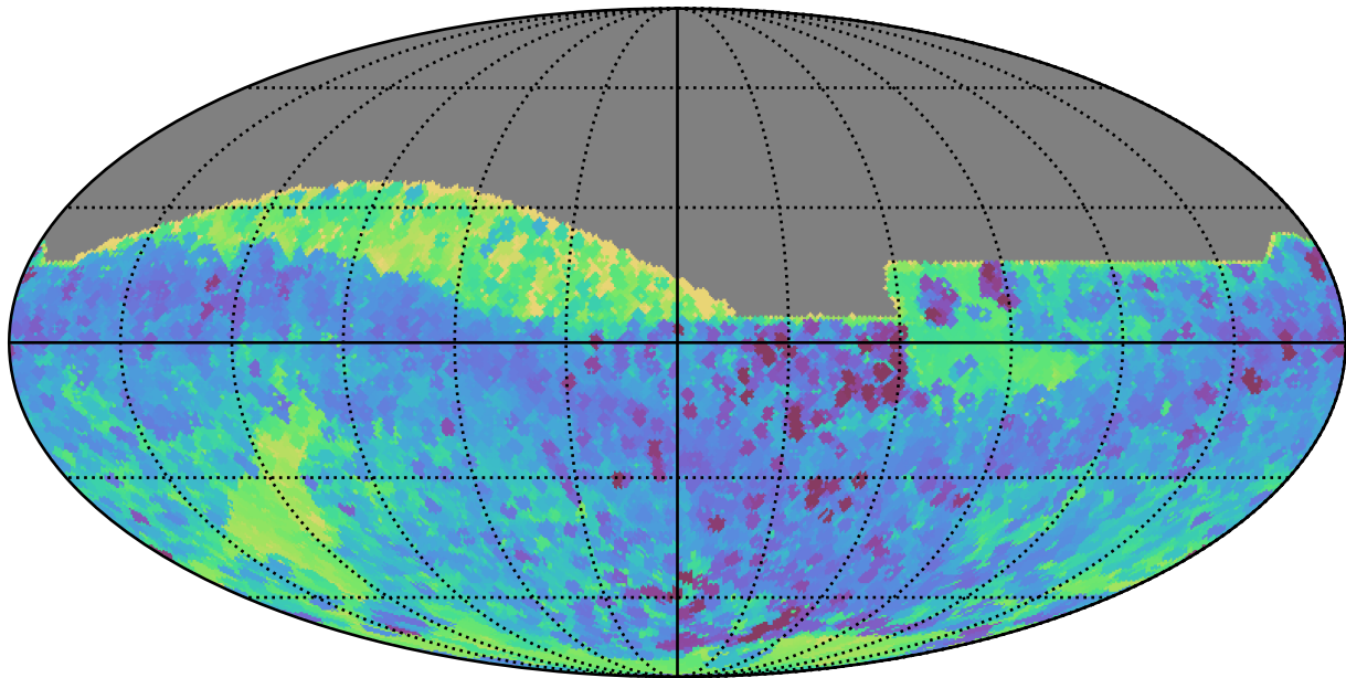
all_long_v3.4_10yrs All sky all bands: Min skyBrightness
