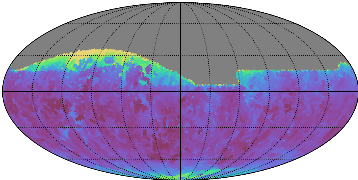
all_long_v3.4_10yrs Yr 1 all bands: Min seeingGeom
