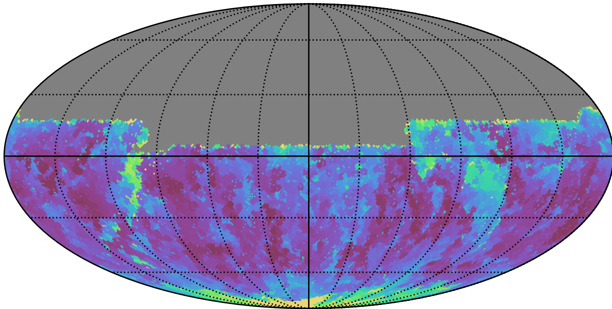
all_long_v3.4_10yrs Yr 1 y band: Min seeingEff
