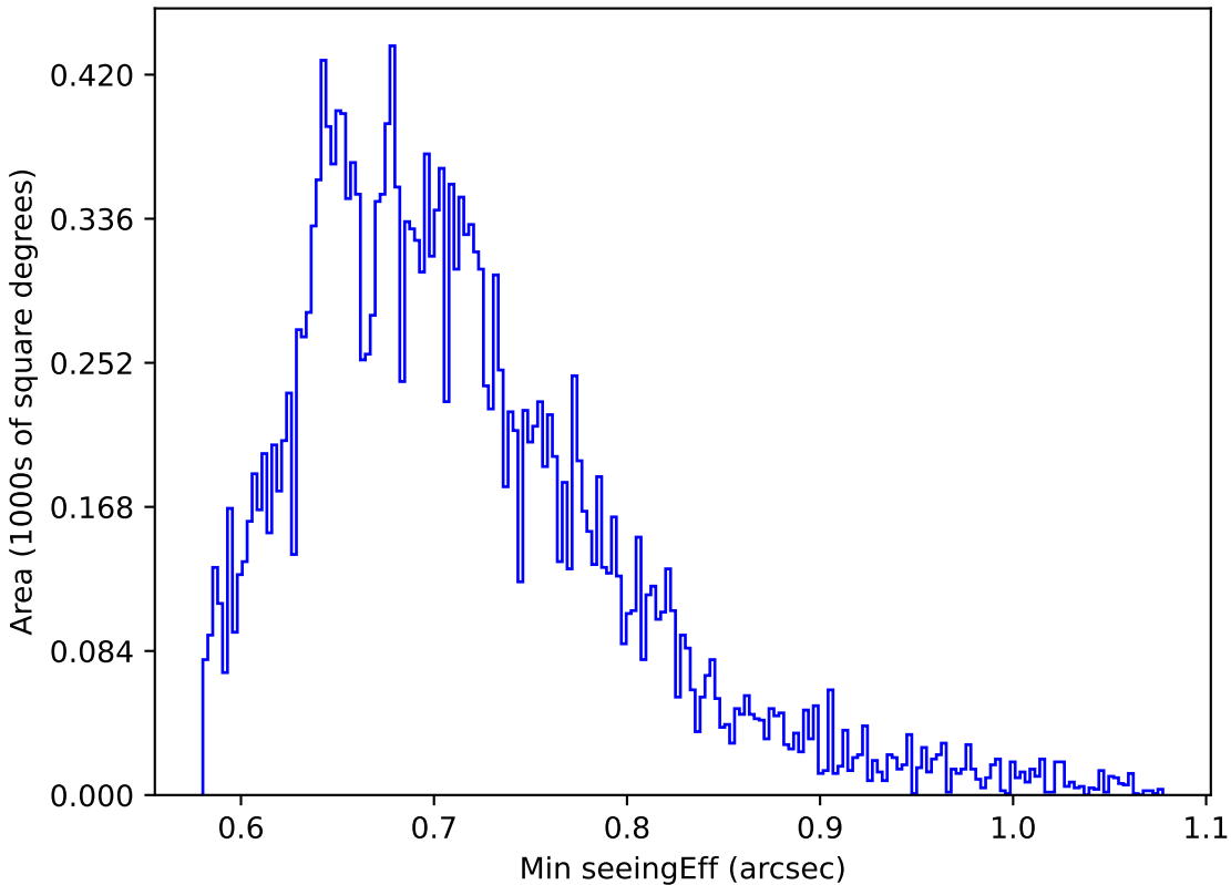
all_long_v3.4_10yrs Yr 1 y band: Min seeingEff
