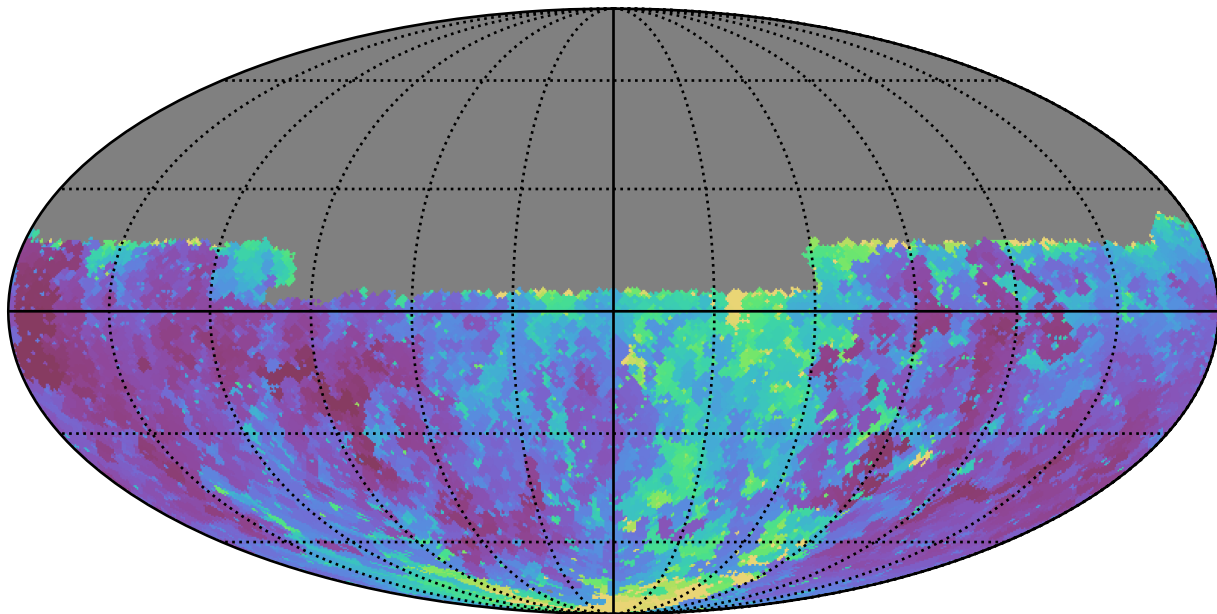
all_long_v3.4_10yrs Yr 1 u band: Min seeingEff
