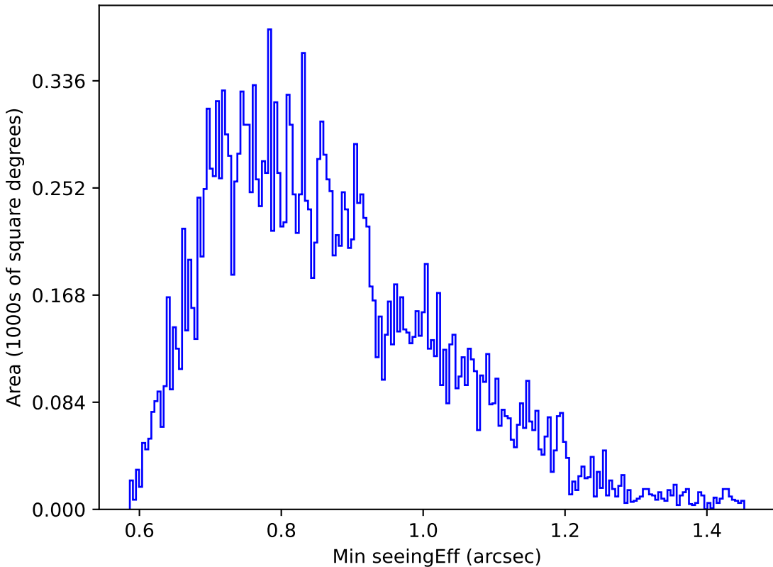
all_long_v3.4_10yrs Yr 1 u band: Min seeingEff
