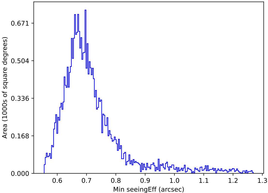
all_long_v3.4_10yrs Yr 1 r band: Min seeingEff
