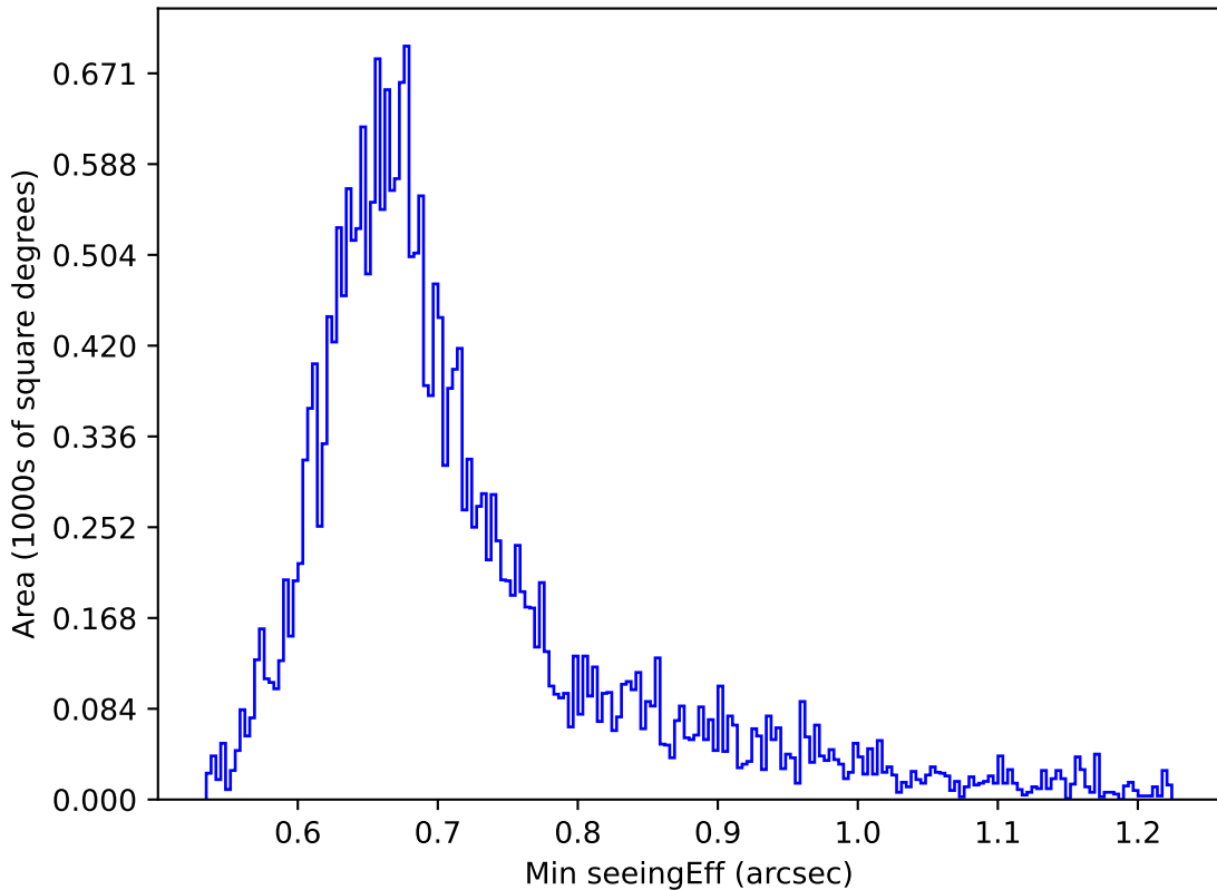
all_long_v3.4_10yrs Yr 1 i band: Min seeingEff
