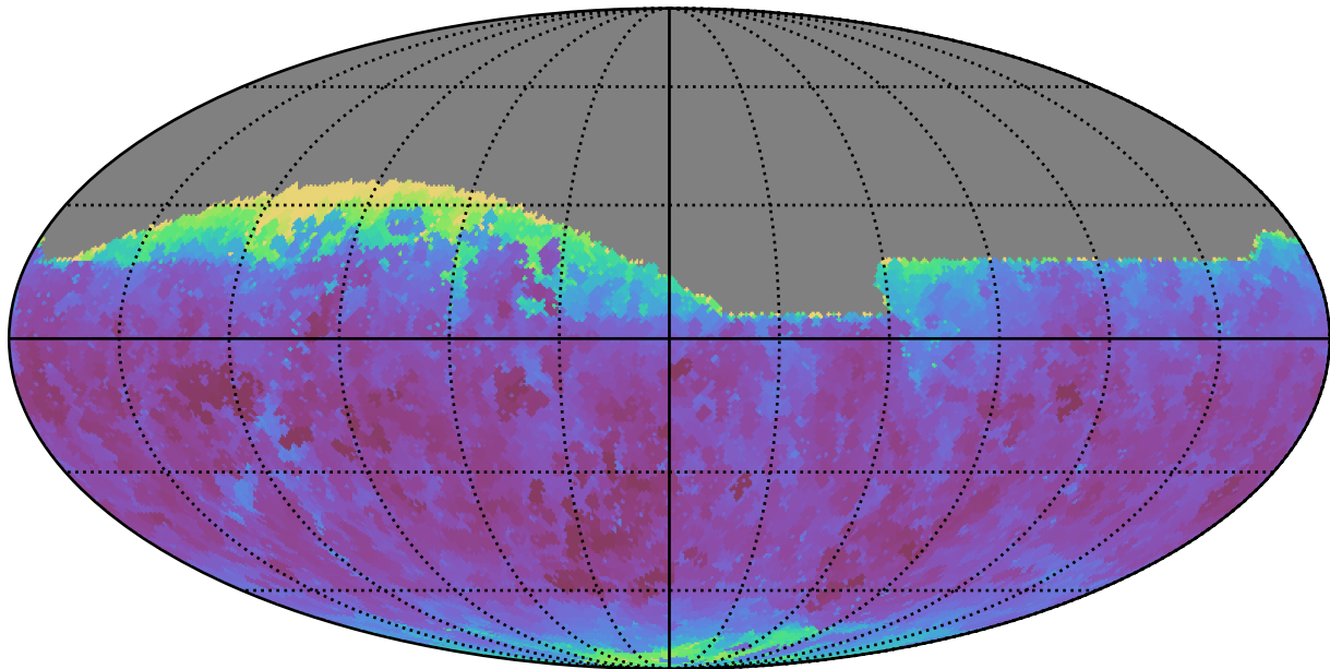
all_long_v3.4_10yrs Yr 1 all bands: Min seeingEff
