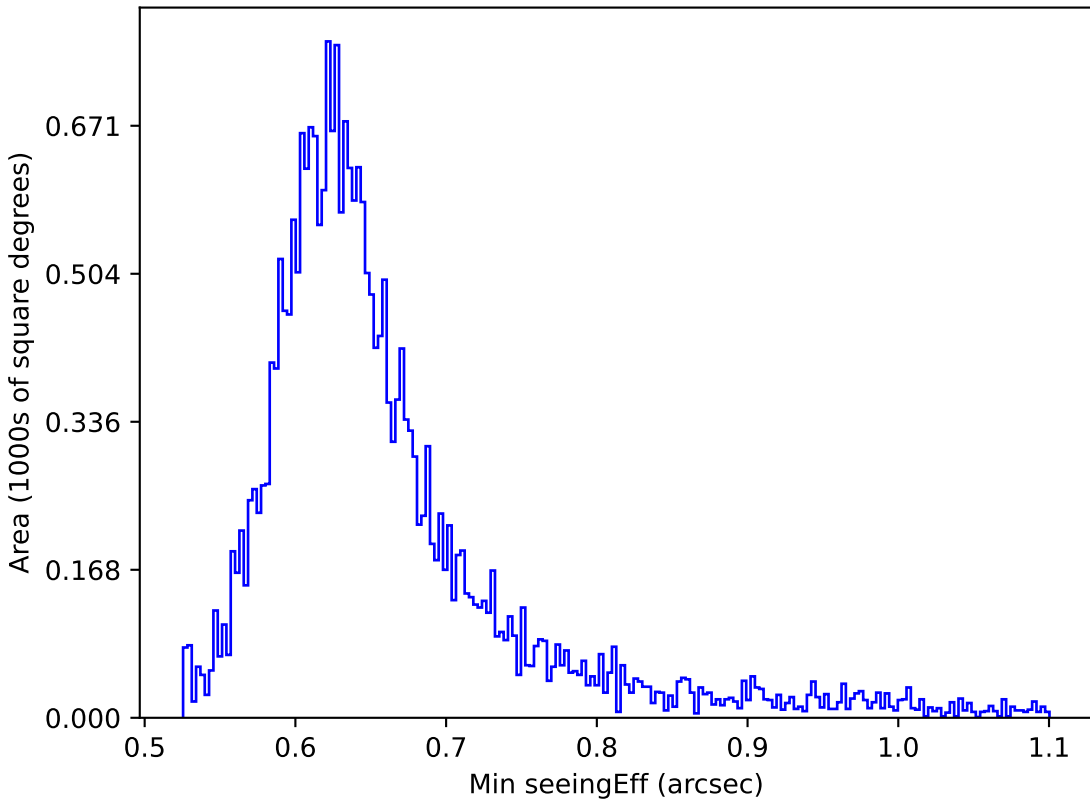
all_long_v3.4_10yrs Yr 1 all bands: Min seeingEff
