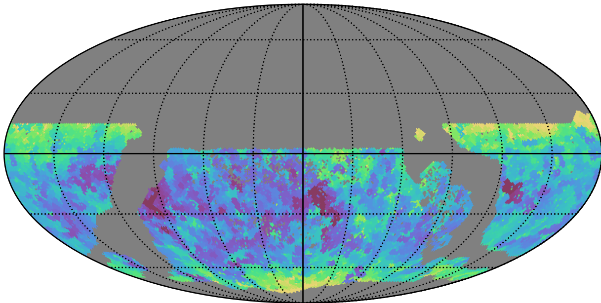
all_long_v3.4_10yrs WFD z band: Min seeingEff
