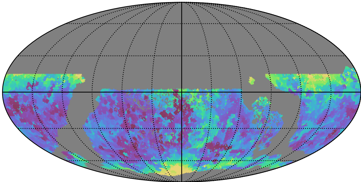
all_long_v3.4_10yrs WFD y band: Min seeingEff
