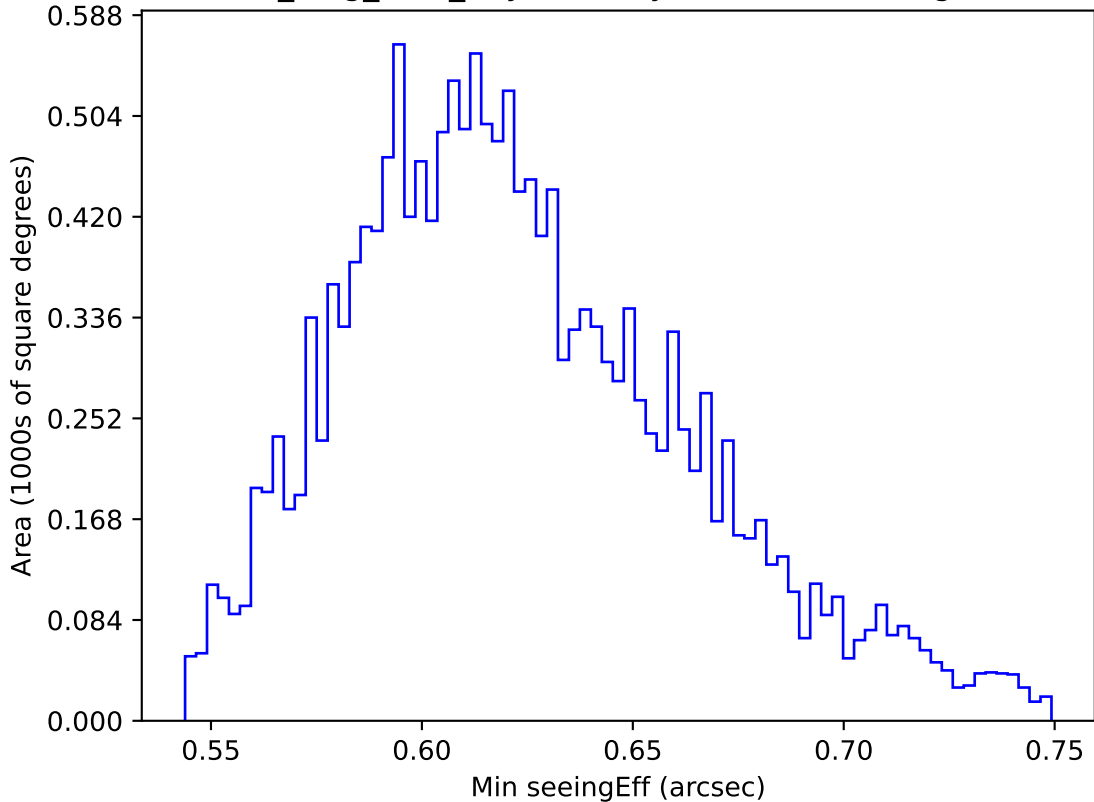
all_long_v3.4_10yrs WFD y band: Min seeingEff
