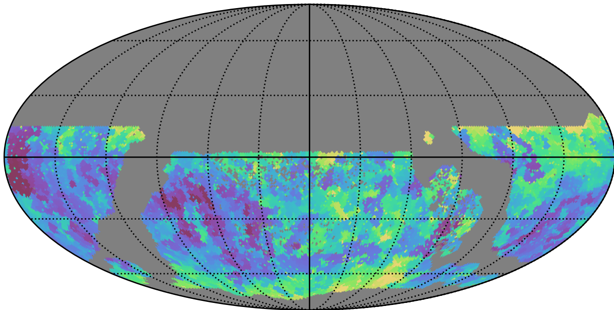
all_long_v3.4_10yrs WFD u band: Min seeingEff
