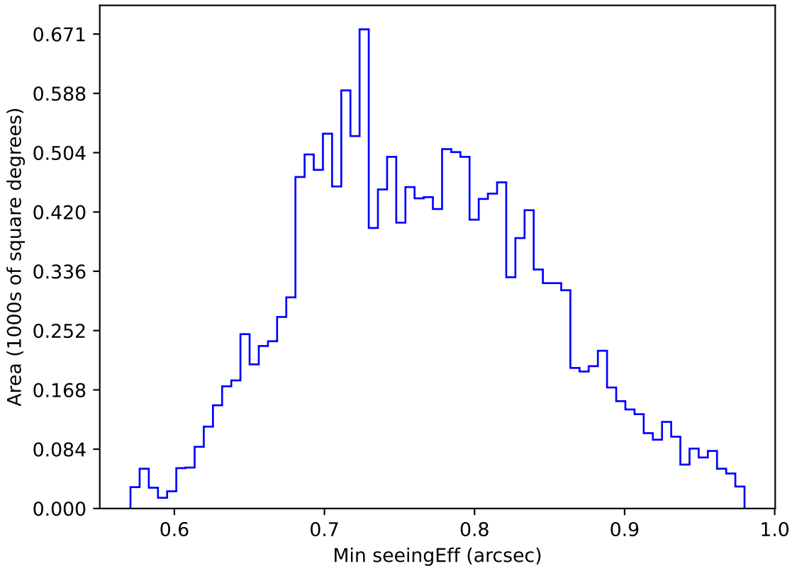
all_long_v3.4_10yrs WFD u band: Min seeingEff
