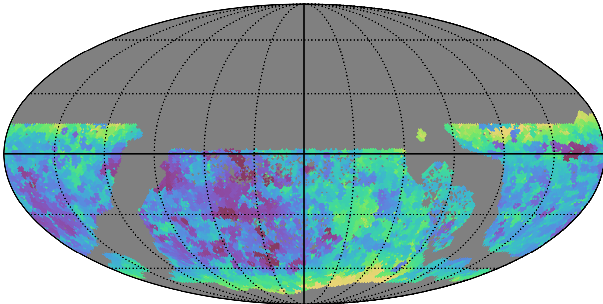
all_long_v3.4_10yrs WFD r band: Min seeingEff
