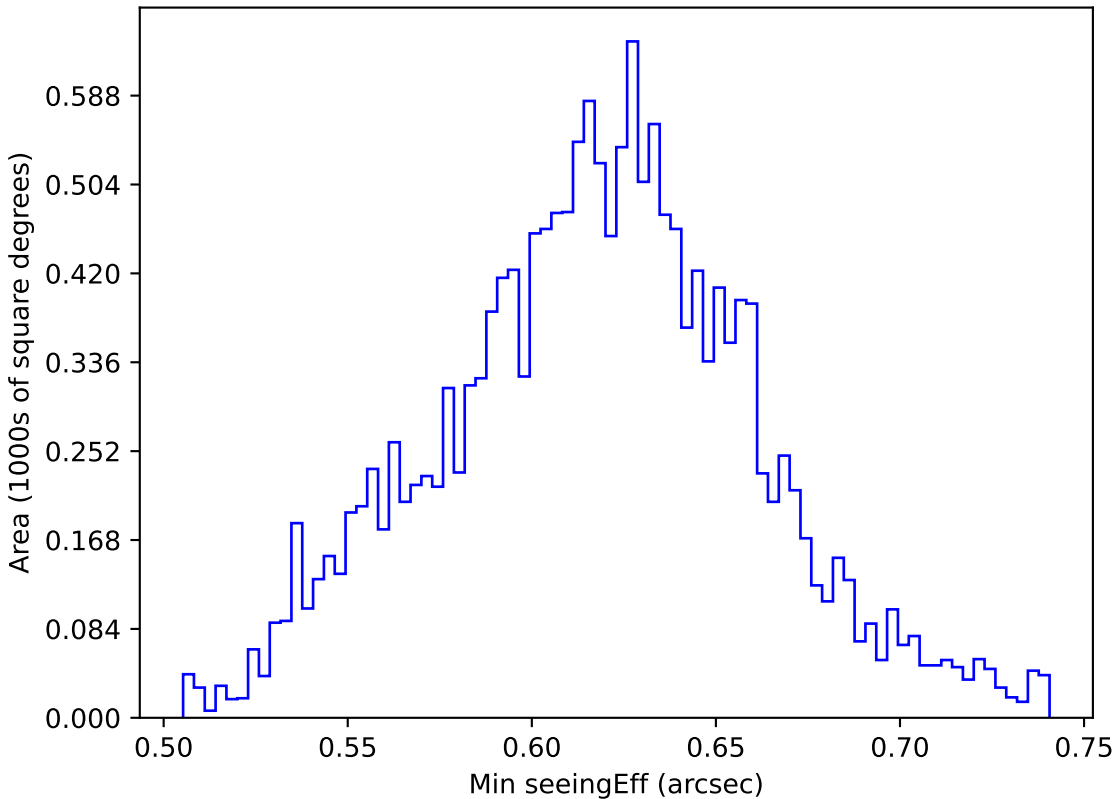
all_long_v3.4_10yrs WFD r band: Min seeingEff
