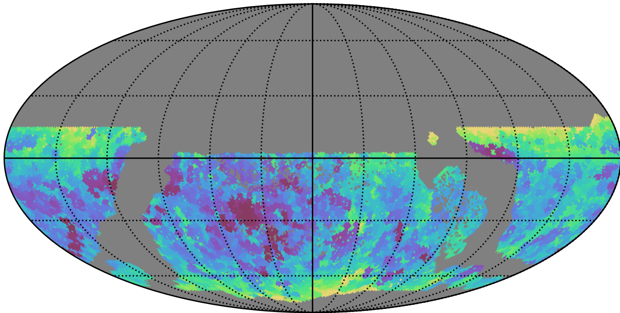
all_long_v3.4_10yrs WFD i band: Min seeingEff
