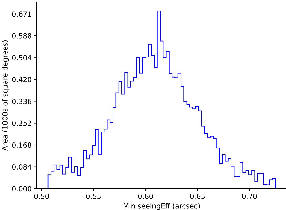
all_long_v3.4_10yrs WFD i band: Min seeingEff
