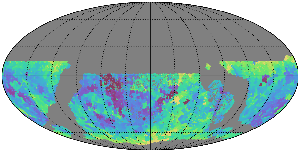
all_long_v3.4_10yrs WFD g band: Min seeingEff
