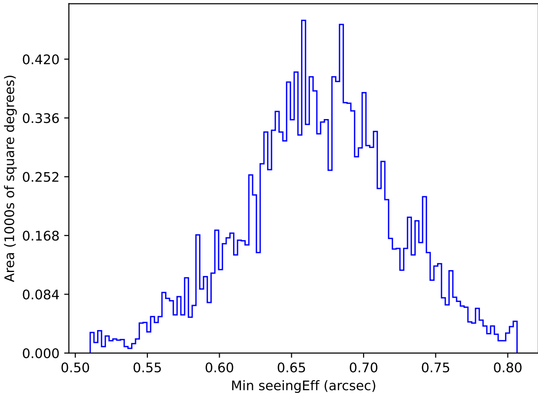
all_long_v3.4_10yrs WFD g band: Min seeingEff
