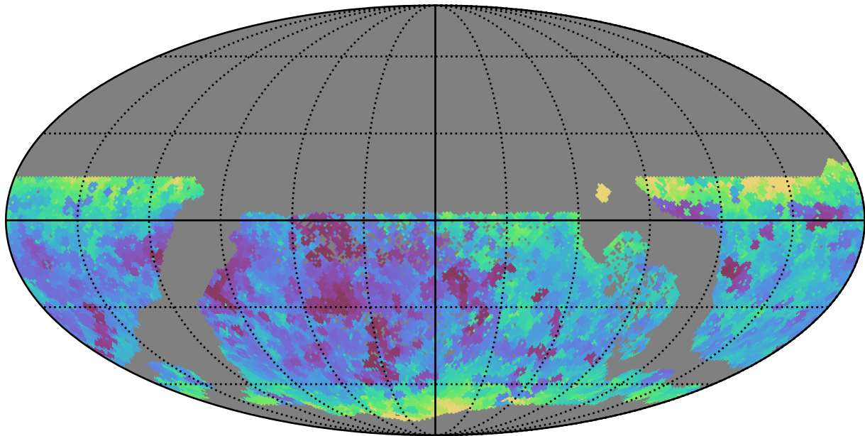
all_long_v3.4_10yrs WFD all bands: Min seeingEff
