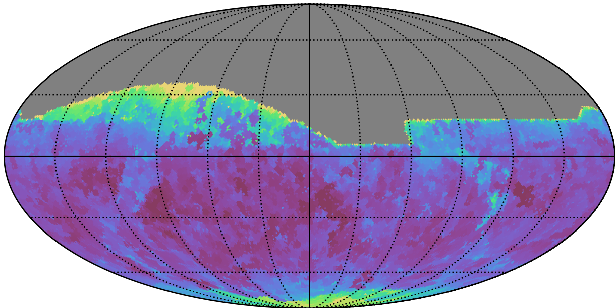
all_long_v3.4_10yrs All sky z band: Min seeingEff
