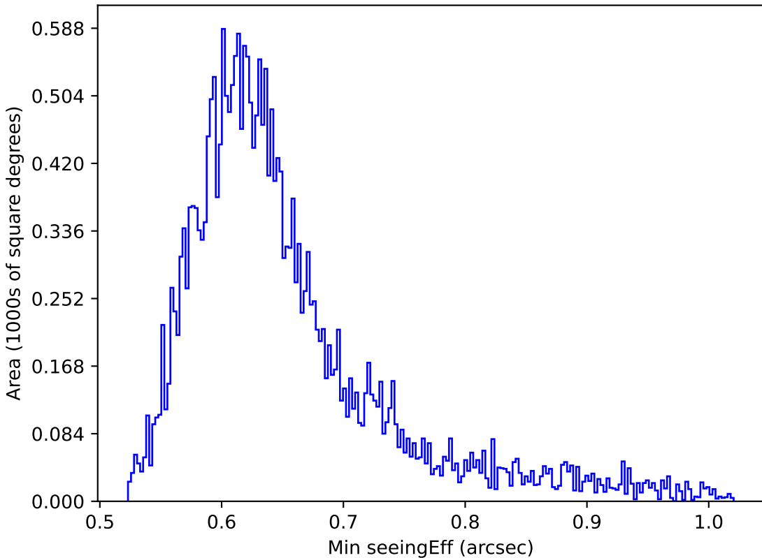
all_long_v3.4_10yrs All sky z band: Min seeingEff
