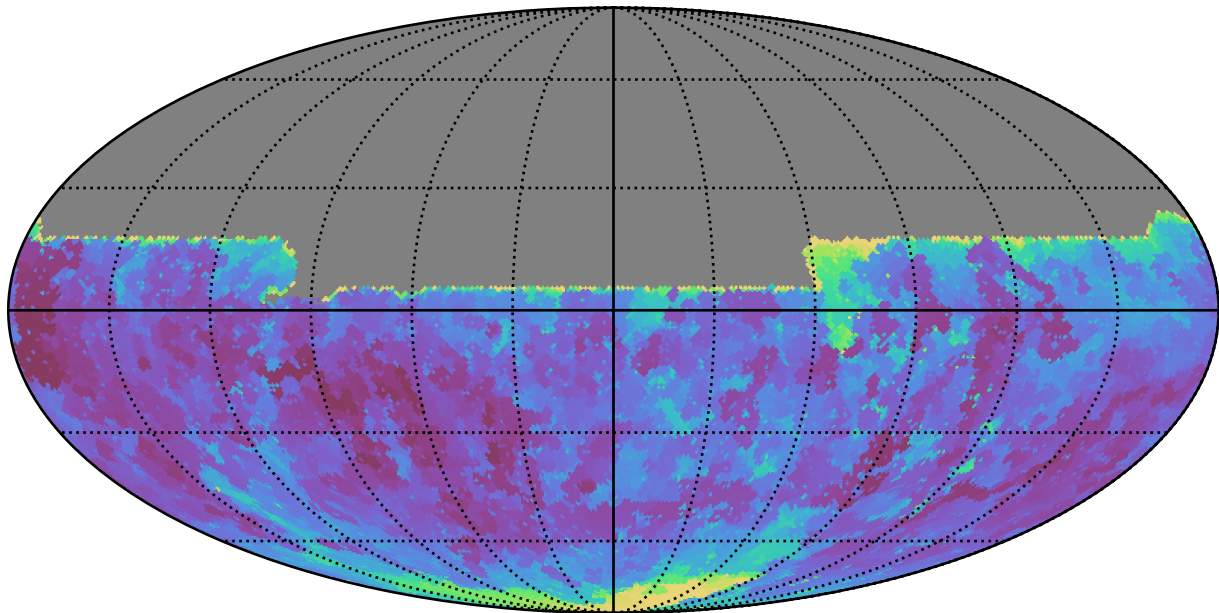
all_long_v3.4_10yrs All sky u band: Min seeingEff
