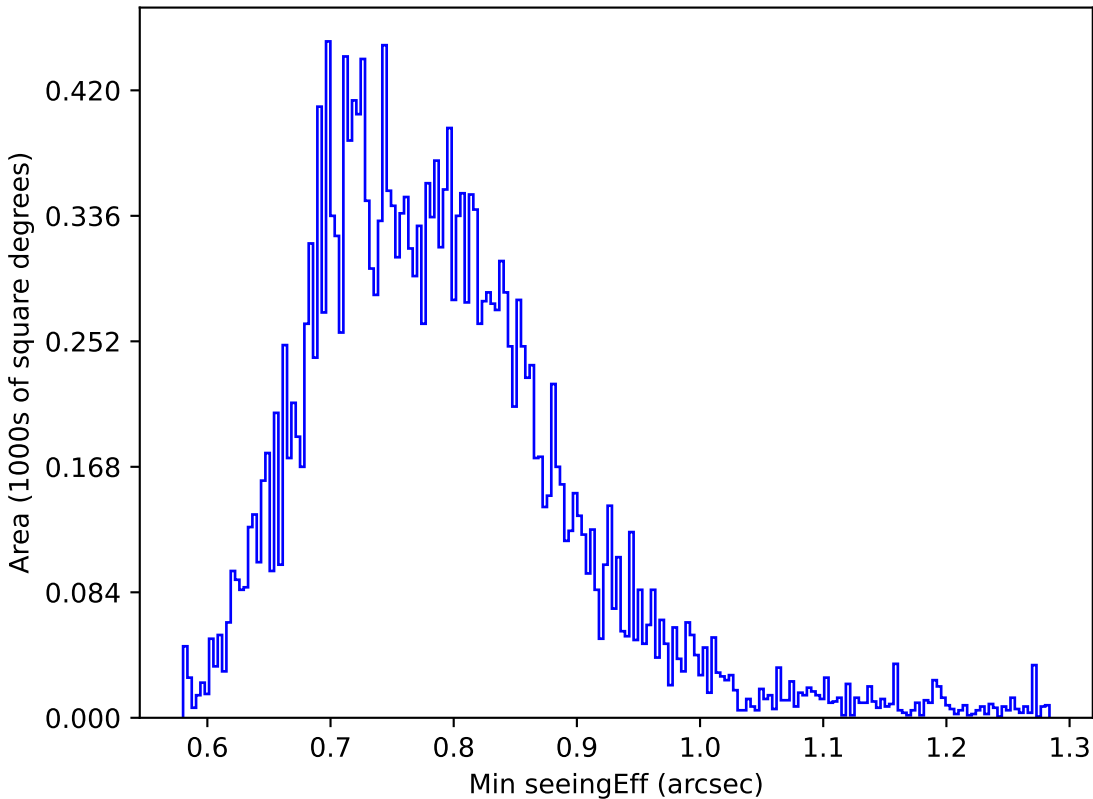
all_long_v3.4_10yrs All sky u band: Min seeingEff
