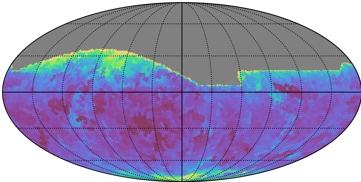
all_long_v3.4_10yrs All sky i band: Min seeingEff
