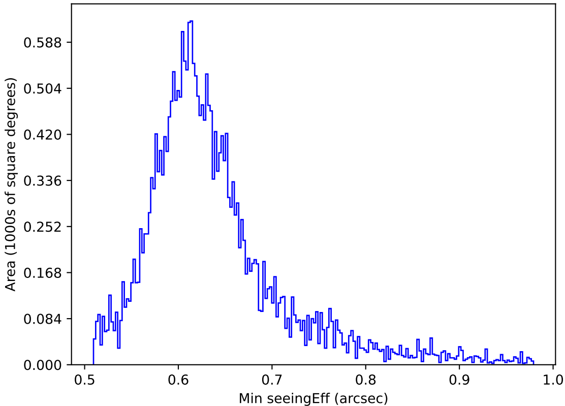
all_long_v3.4_10yrs All sky i band: Min seeingEff
