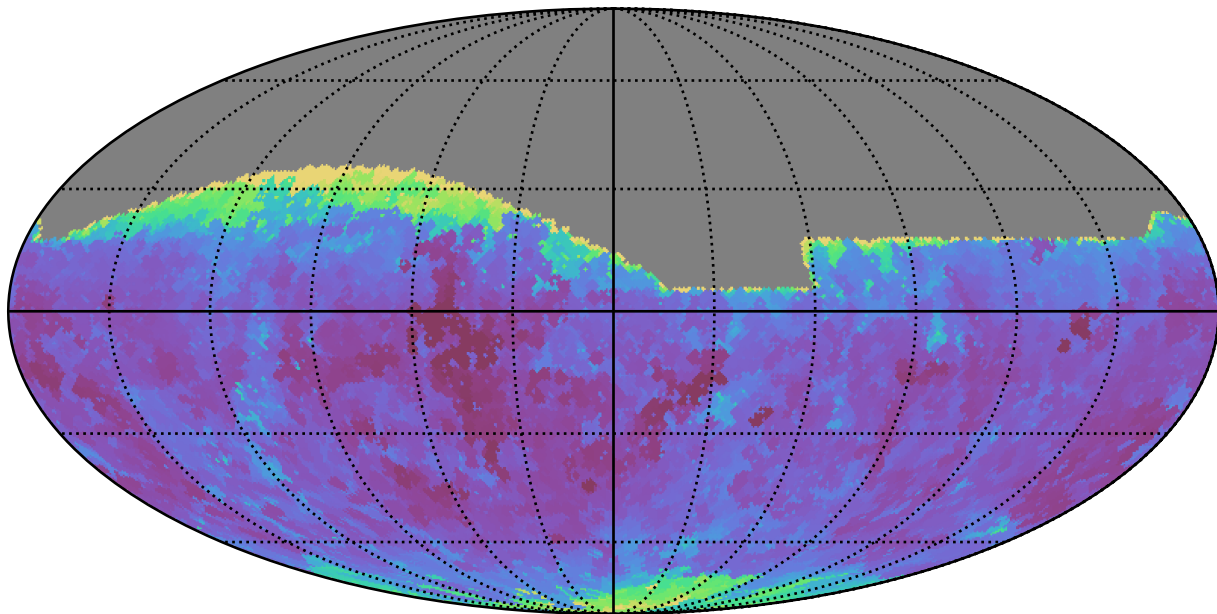
all_long_v3.4_10yrs All sky g band: Min seeingEff
