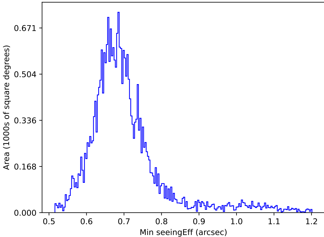
all_long_v3.4_10yrs All sky g band: Min seeingEff
