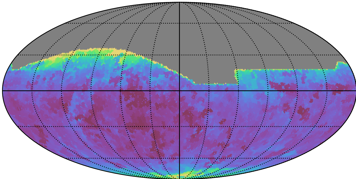
all_long_v3.4_10yrs All sky all bands: Min seeingEff
