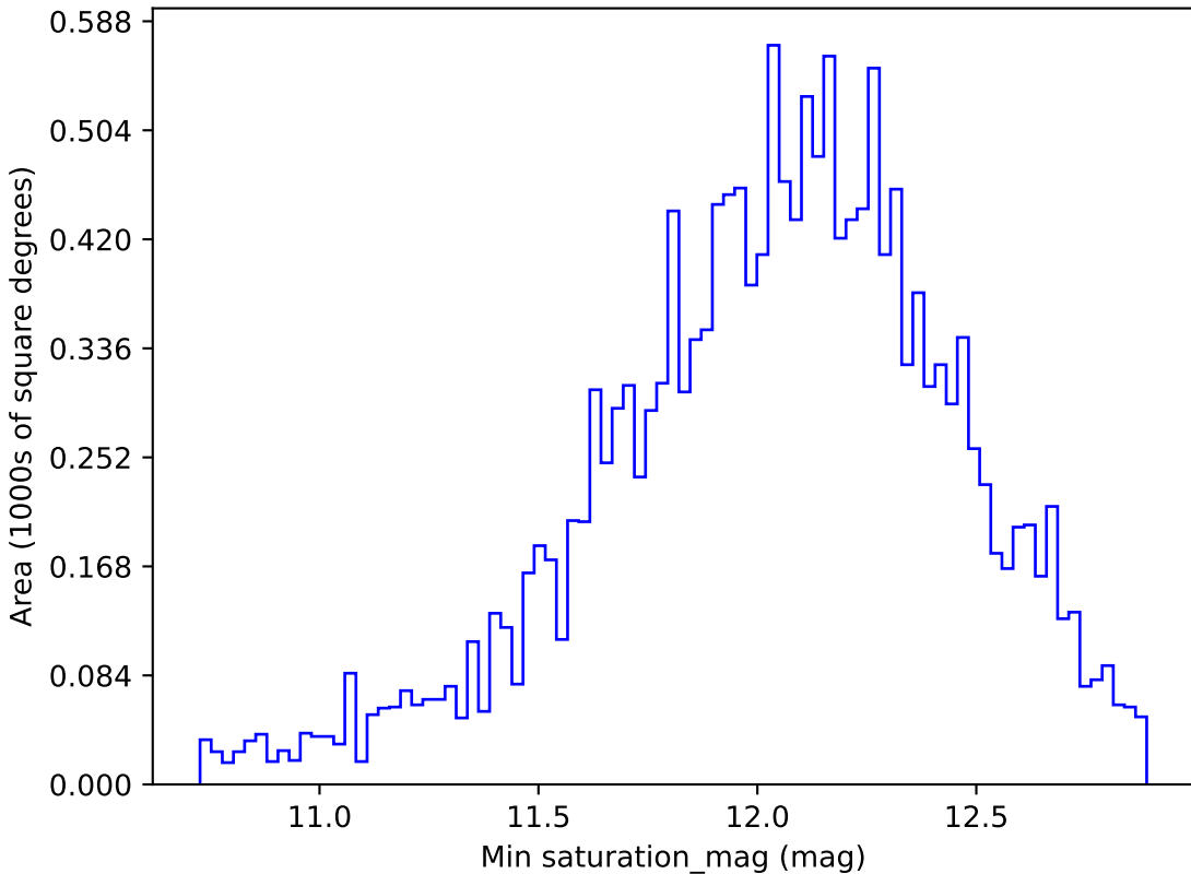
all_long_v3.4_10yrs WFD z band: Min saturation_mag
