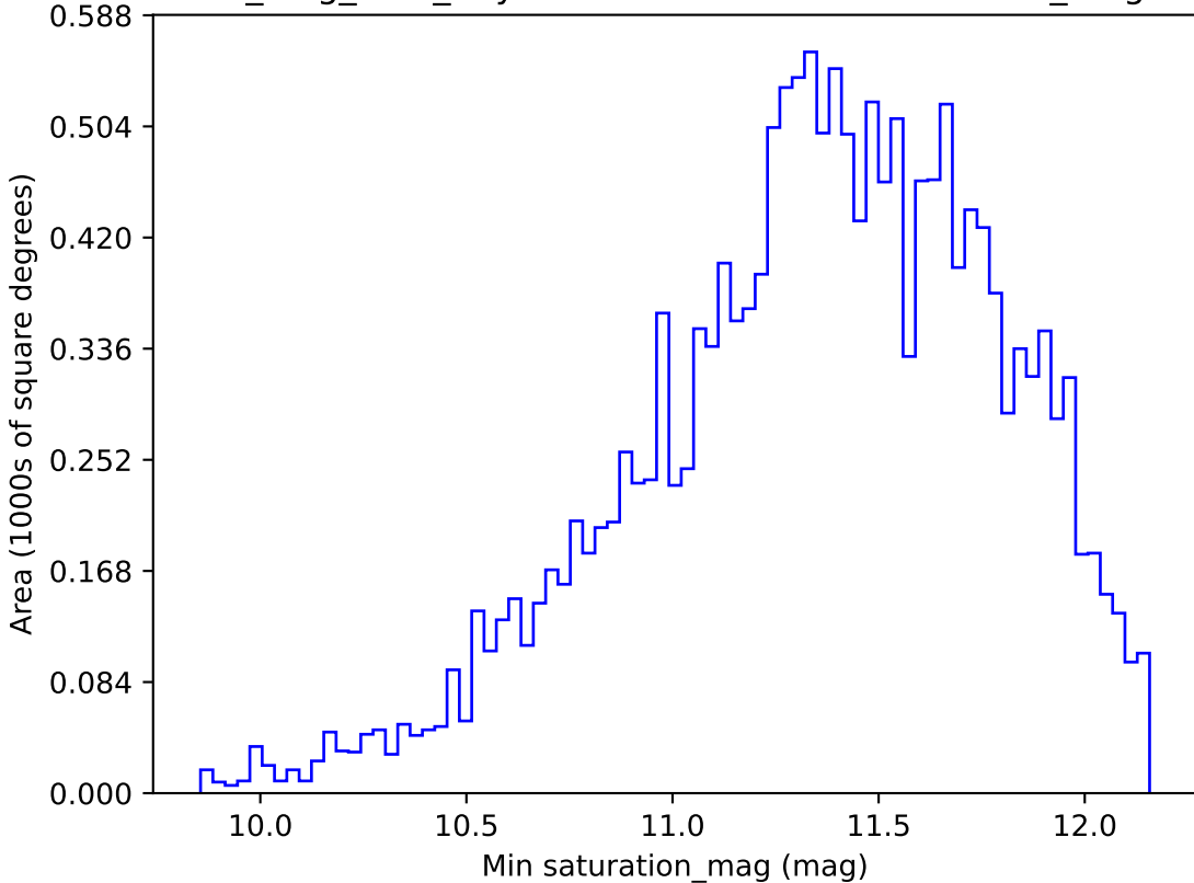
all_long_v3.4_10yrs WFD u band: Min saturation_mag
