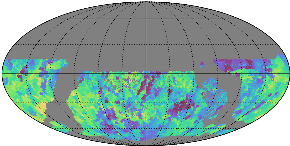
all_long_v3.4_10yrs WFD r band: Min saturation_mag
