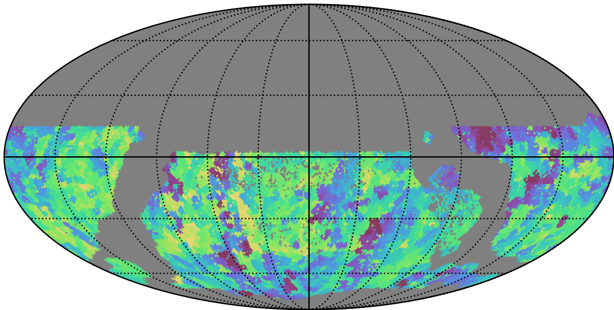
all_long_v3.4_10yrs WFD g band: Min saturation_mag
