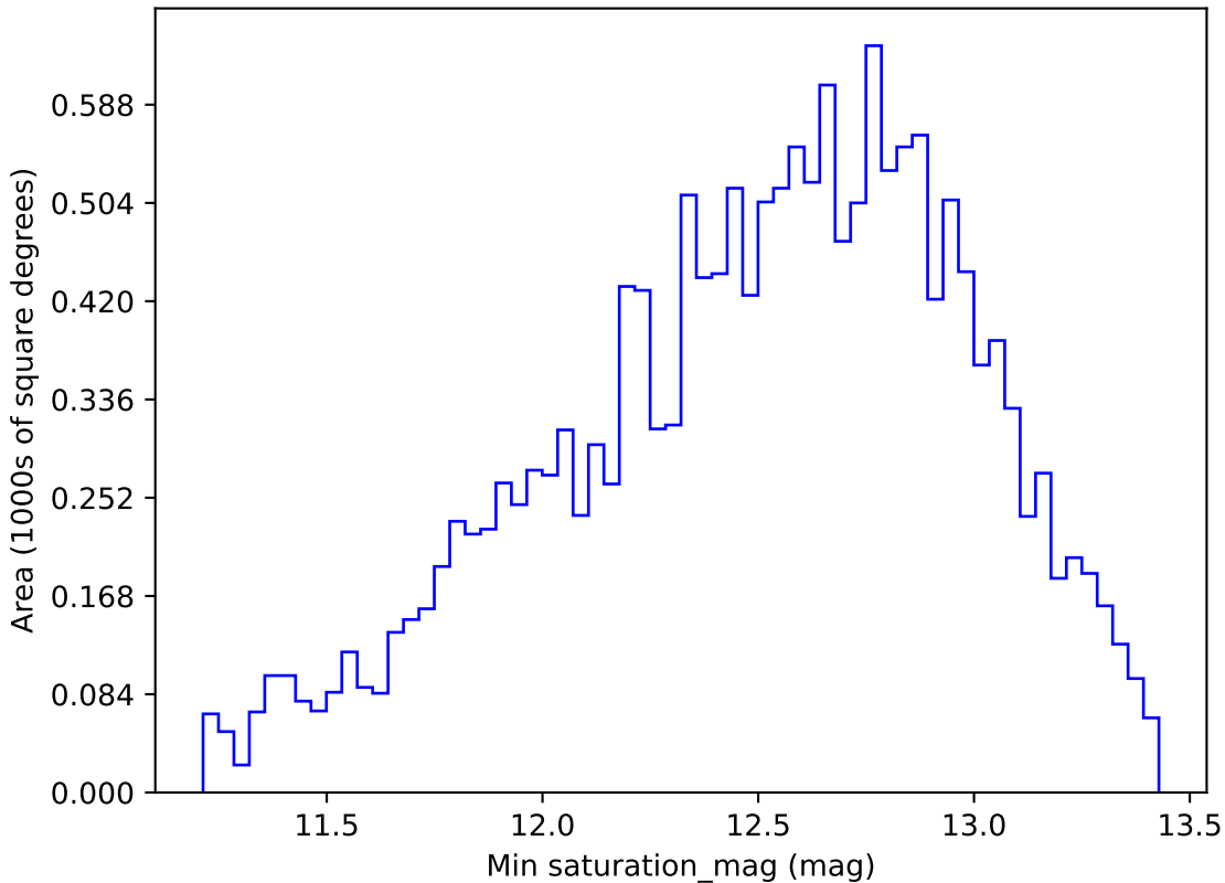
all_long_v3.4_10yrs WFD g band: Min saturation_mag
