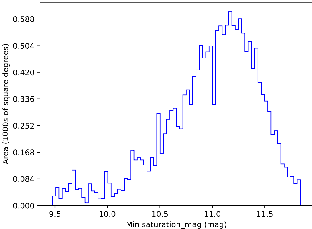
all_long_v3.4_10yrs WFD all bands: Min saturation_mag
