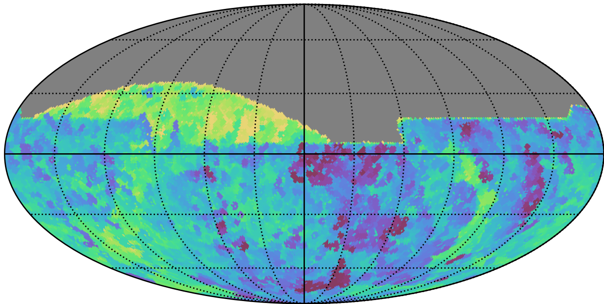
all_long_v3.4_10yrs All sky all bands: Min saturation_mag
