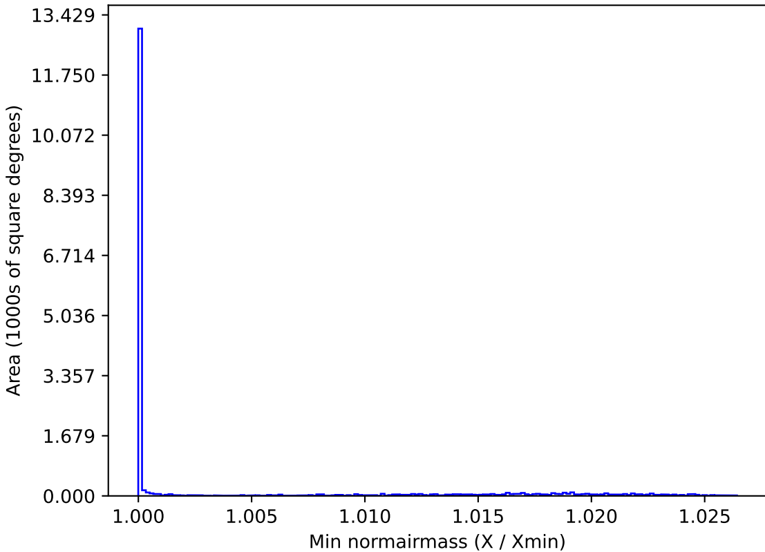
all_long_v3.4_10yrs WFD all bands: Min normairmass
