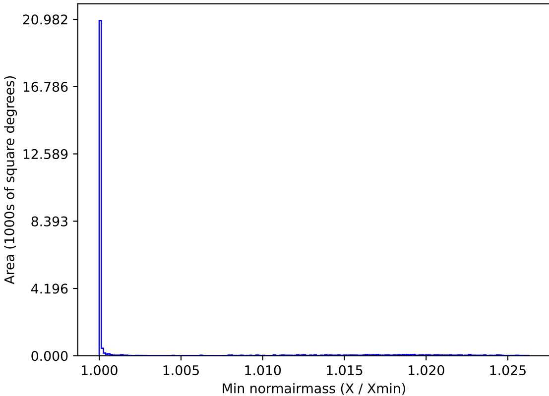
all_long_v3.4_10yrs All sky all bands: Min normairmass
