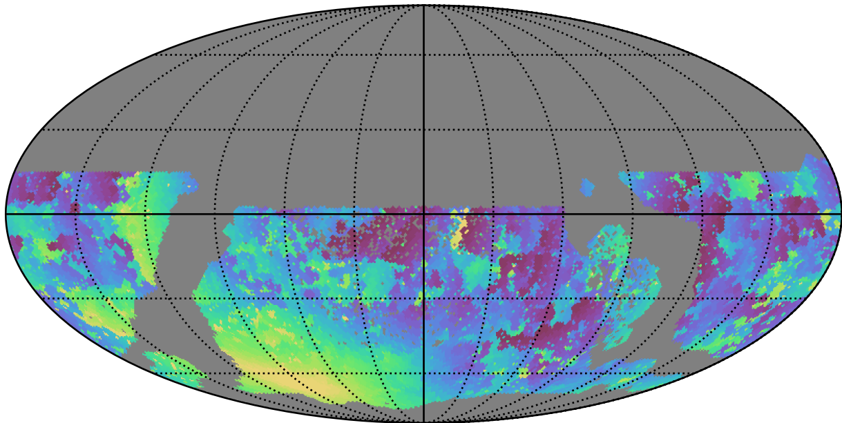
all_long_v3.4_10yrs WFD u band: Min moonDistance
