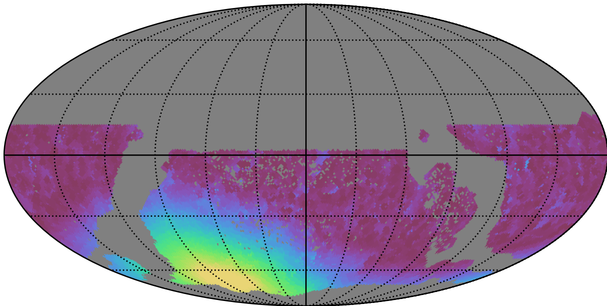
all_long_v3.4_10yrs WFD r band: Min moonDistance
