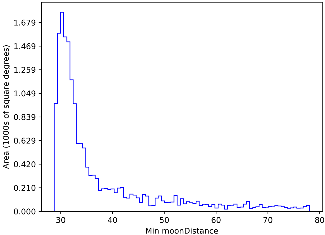
all_long_v3.4_10yrs WFD r band: Min moonDistance
