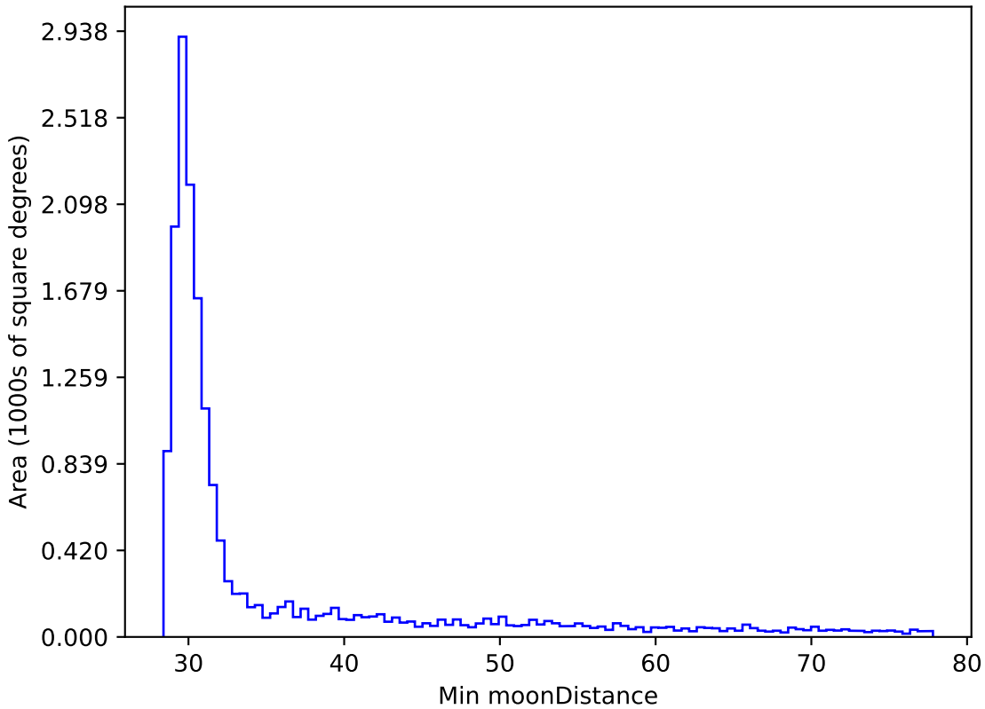
all_long_v3.4_10yrs WFD i band: Min moonDistance
