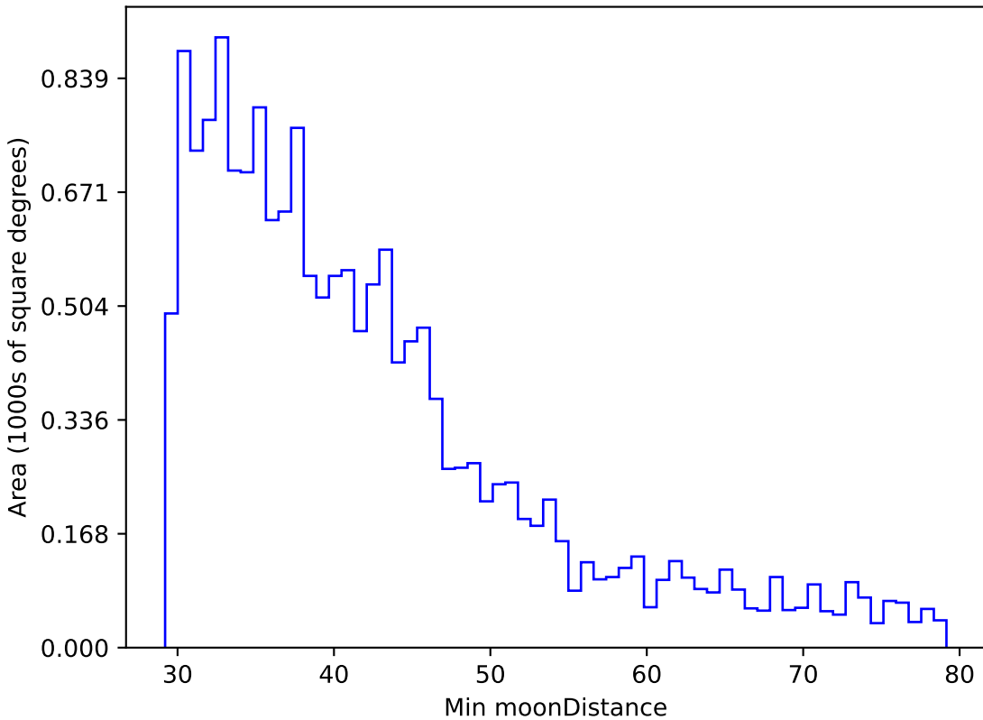
all_long_v3.4_10yrs WFD g band: Min moonDistance
