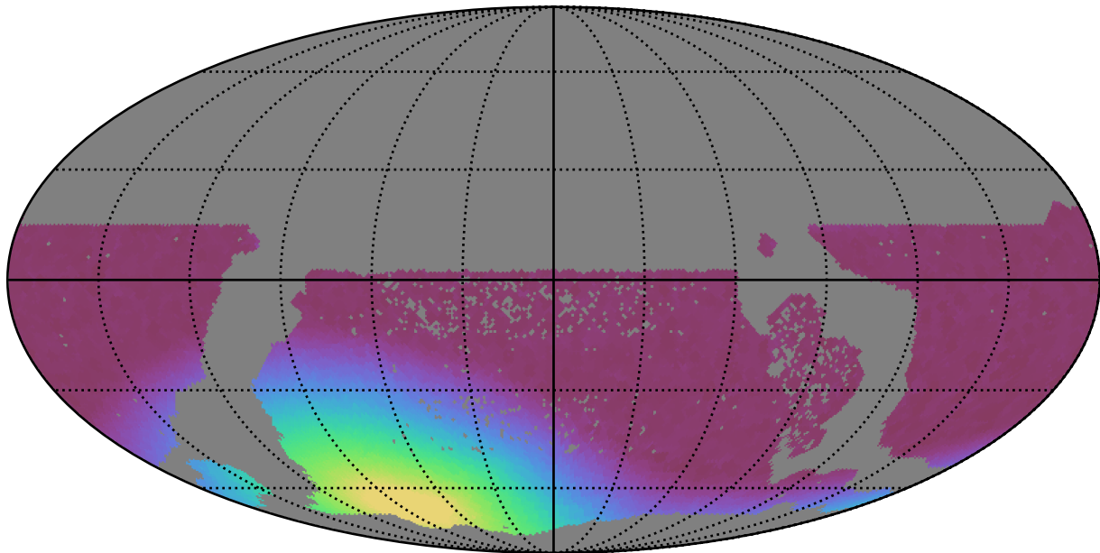
all_long_v3.4_10yrs WFD all bands: Min moonDistance
