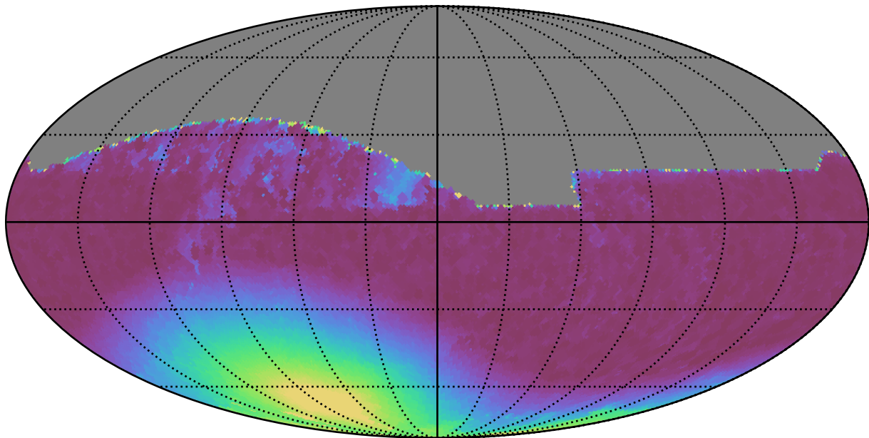
all_long_v3.4_10yrs All sky z band: Min moonDistance
