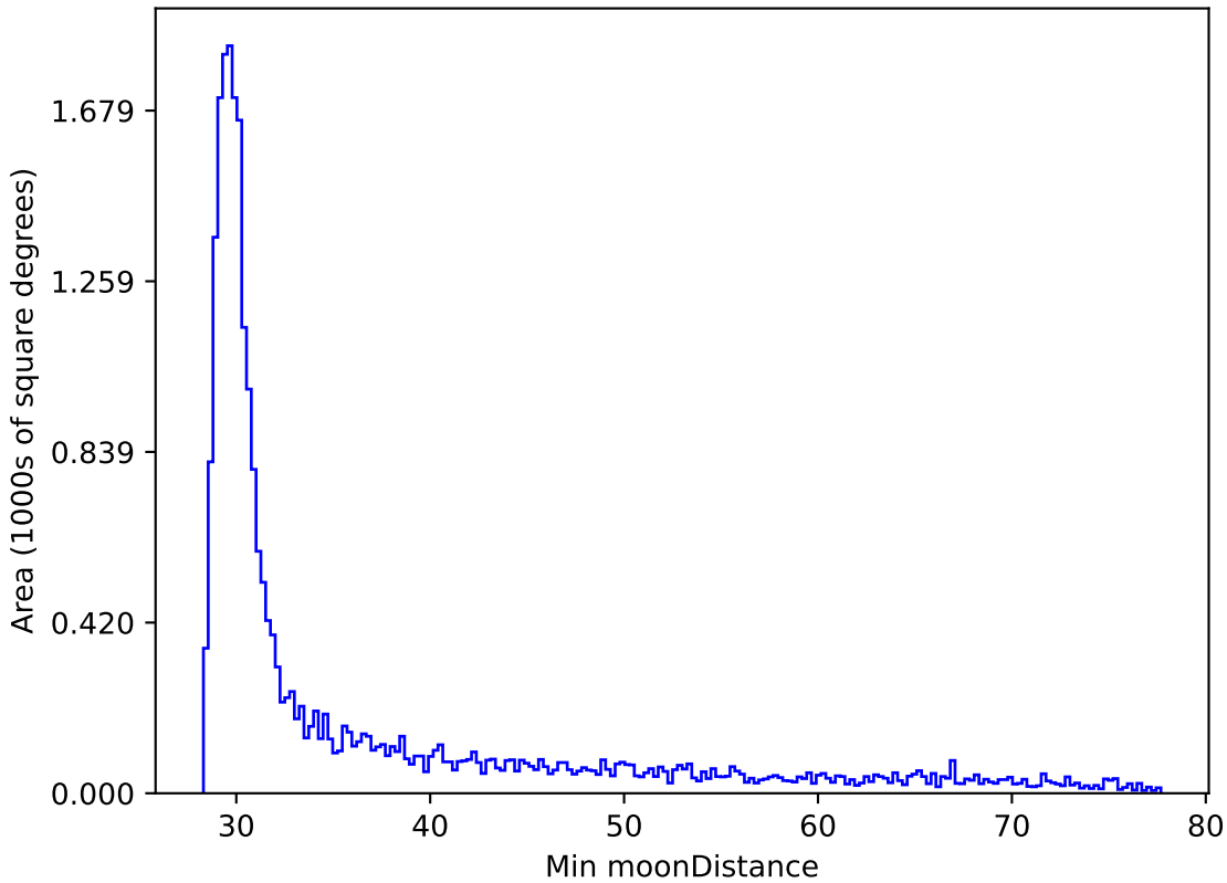
all_long_v3.4_10yrs All sky z band: Min moonDistance
